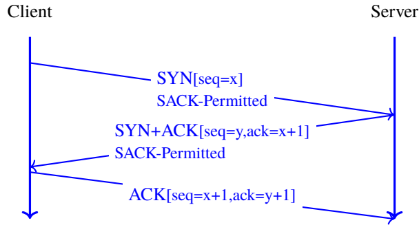
Fig. 2.2: Negotiating the utilization of Selective Acknowledgments during the three-way handshake
