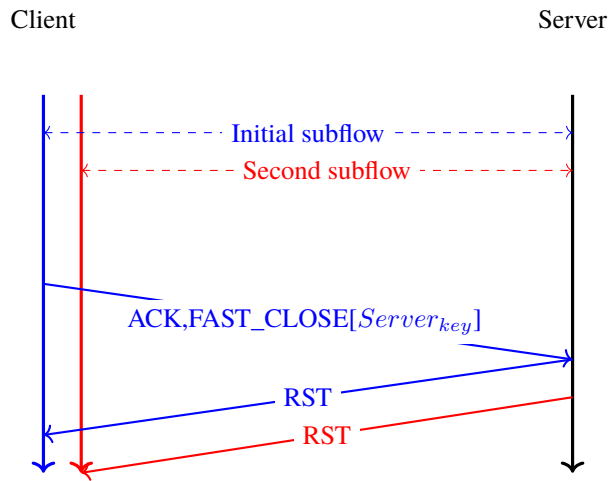
Fig. 3.23: Abrupt release of a Multipath TCP connection by sending FAST_CLOSE inside an ACK
