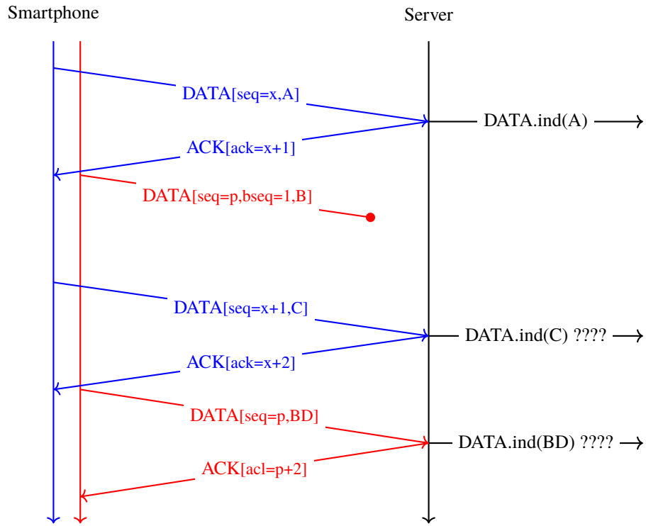
Fig. 3.8: A naive approach to send data over a Multipath TCP connection
