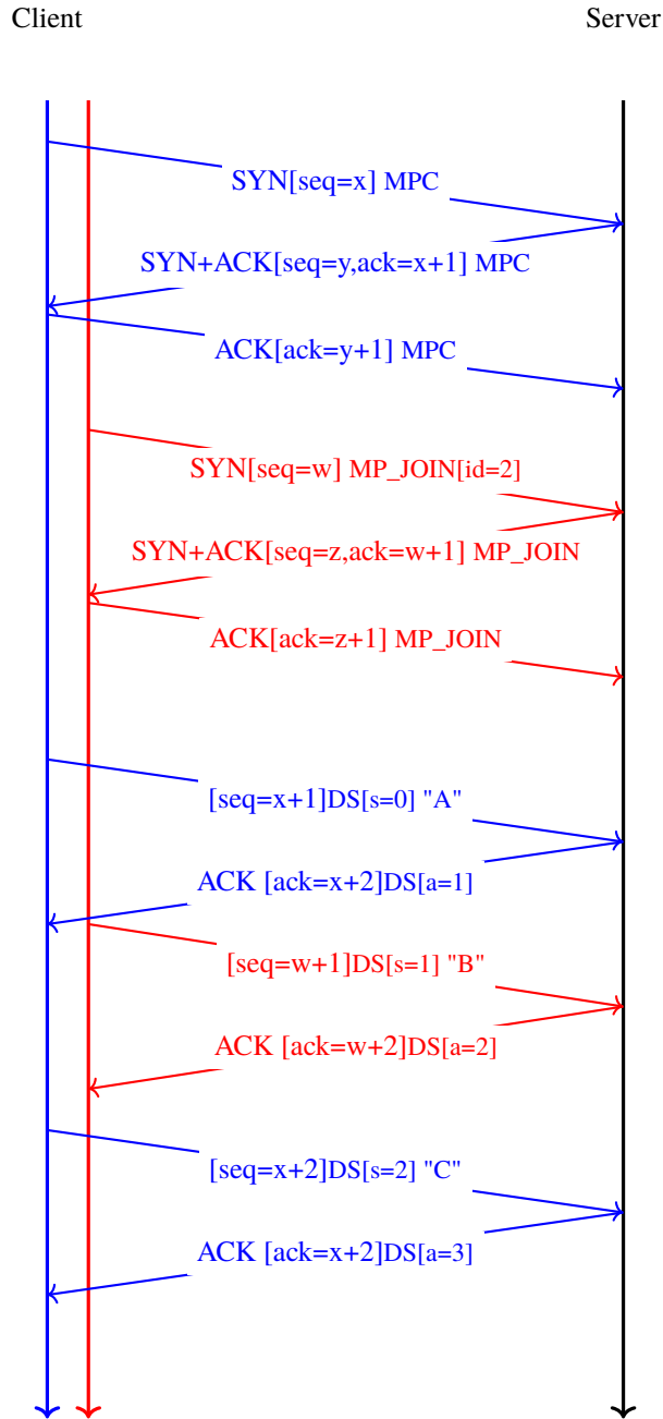
Fig. 3.18: Multipath TCP relies on data sequence numbers and acknowledgments
