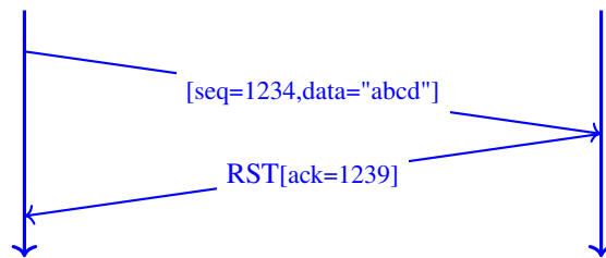
Fig. 2.9: Closing a TCP connection using a RST segment
