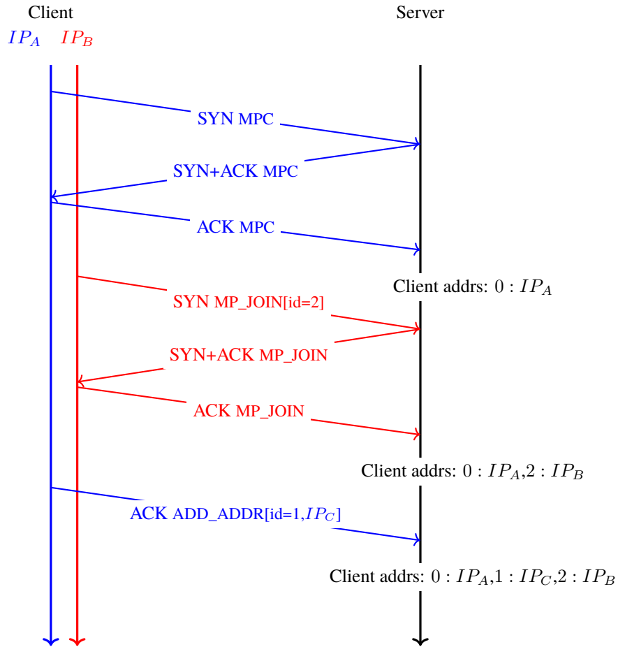
Fig. 3.16: A Multipath TCP hosts remembers the addresses used by its peer
