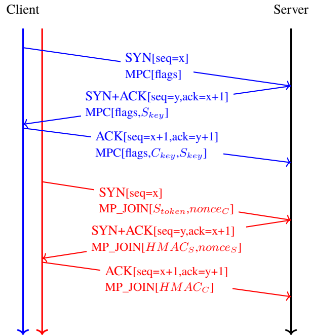
Fig. 3.14: A client creates a second subflow by creating a TCP connection with the MP_JOIN option
