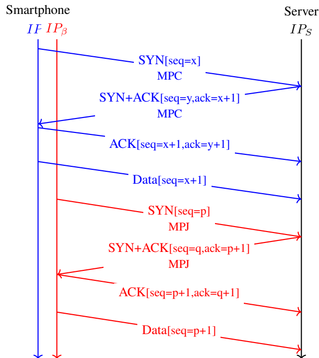
Fig. 3.3: A Multipath TCP connection with two subflows
