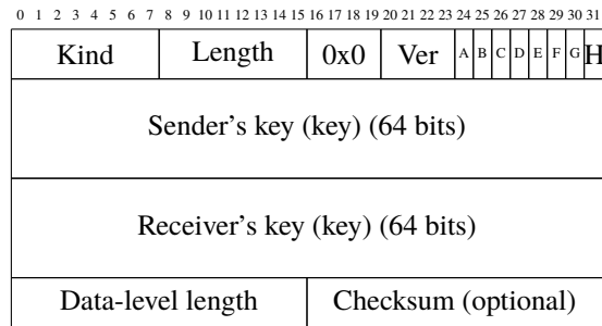
Fig. 3.43: The MP_CAPABLE option in initiator's first ACK (with data)
