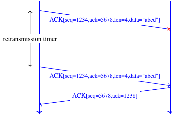
Fig. 2.6: TCP protects data by a retransmission timer
