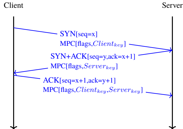
Fig. 3.13: Negotiating the utilization of Multipath TCP version 0
