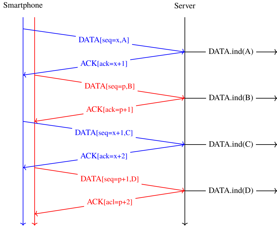
Fig. 3.7: A naive approach to send data over a Multipath TCP connection
