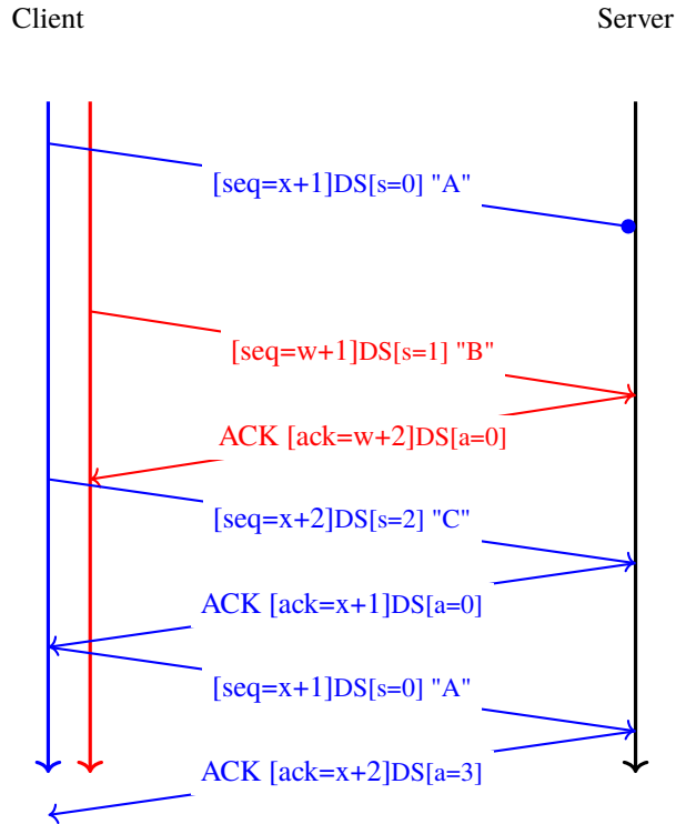
Fig. 3.19: Multipath TCP copes with packet losses
