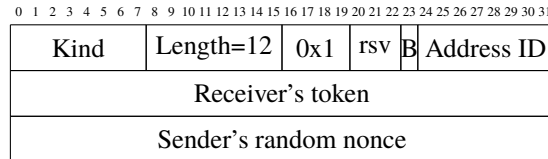
Fig. 3.33: The MP_JOIN option in a SYN packet
