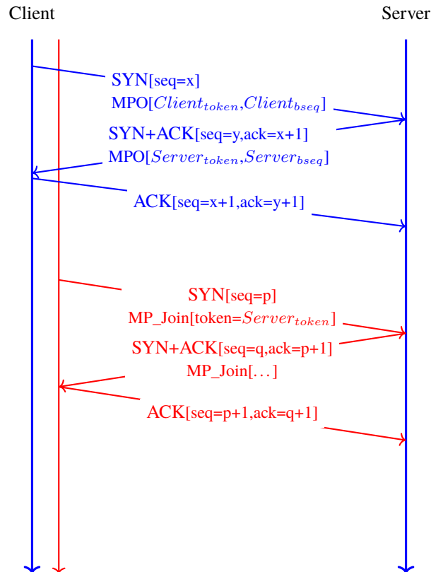
Fig. 3.10: Opening a Multipath TCP connection with a MPO option
