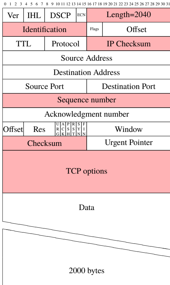
Fig. 3.31: A large IP packet containing TCP header and data
