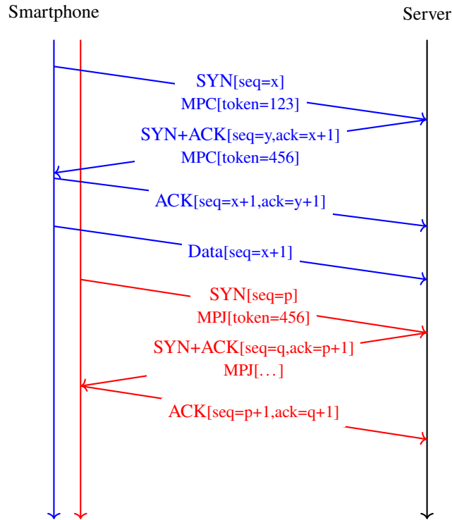
Fig. 3.5: The tokens exchanged during the handshake allow to associate subsequent subflows to existing Multipath TCP connections
