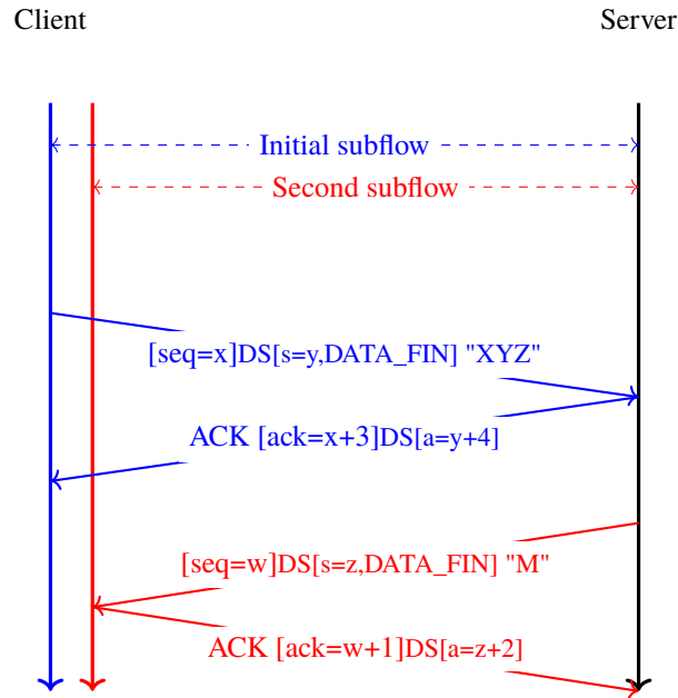
Fig. 3.22: Graceful termination of a Multipath TCP connection
