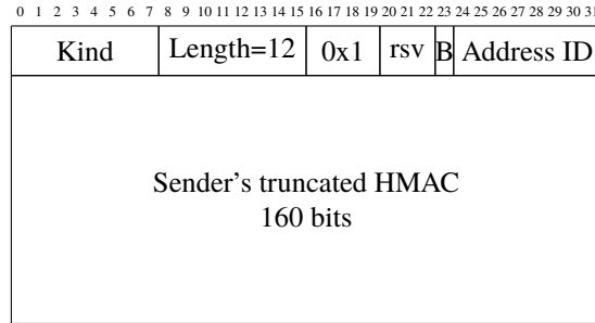
Fig. 3.35: The MP_JOIN option in the initiator's first ACK
