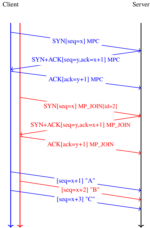
Fig. 3.17: A naive approach to exchange data over different subflows
