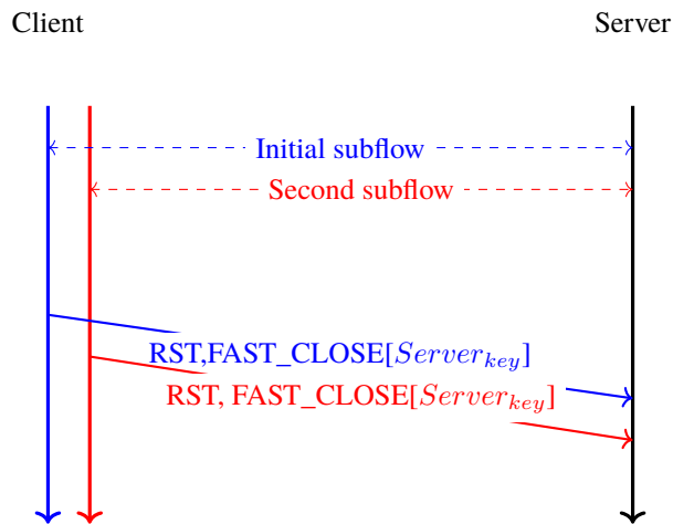
Fig. 3.24: Abrupt release of a Multipath TCP connection by sending a RST with FAST_CLOSE on all subflows
