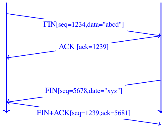
Fig. 2.8: Closing a TCP connection using the FIN flag
