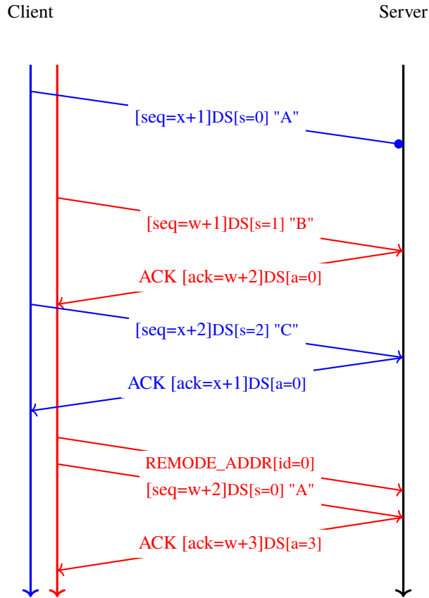
Fig. 3.20: Multipath TCP copes with subflow failures
