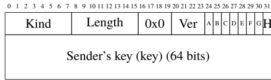
Fig. 3.41: The MP_CAPABLE option in SYN+ACK packet
