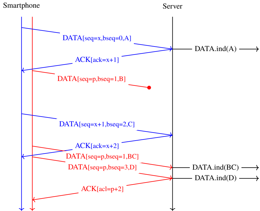
Fig. 3.9: A naive approach to send data over a Multipath TCP connection
