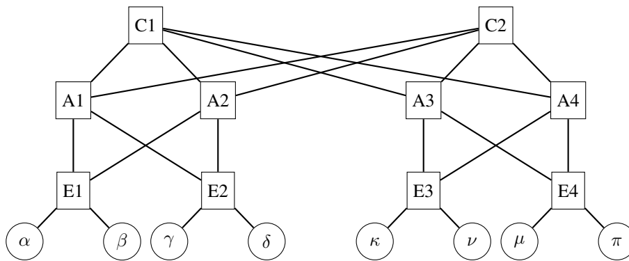
Fig. 3.6: A simple datacenter network
