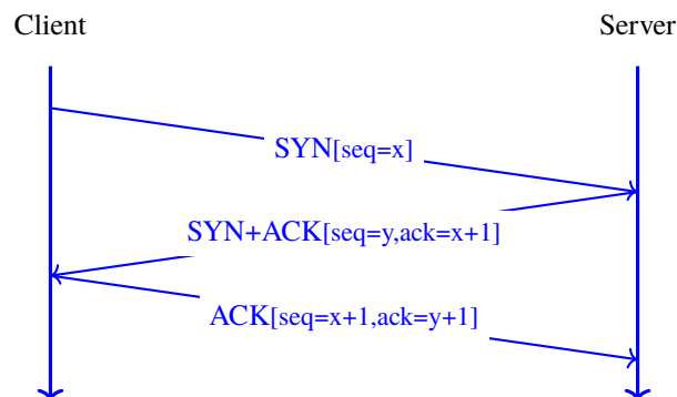
Fig. 2.1: Establishing a TCP connection using the three-way handshake
