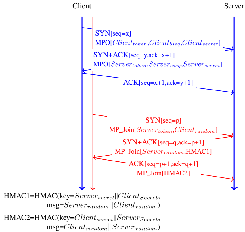
Fig. 3.11: Creating a Multipath TCP connection with a MPO option
