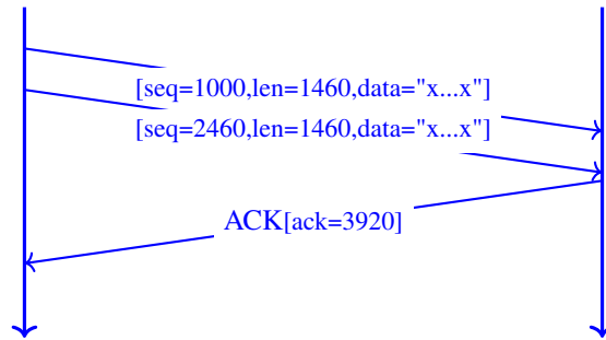
Fig. 2.4: TCP Reliable data transfer with delayed acknowledgments.
