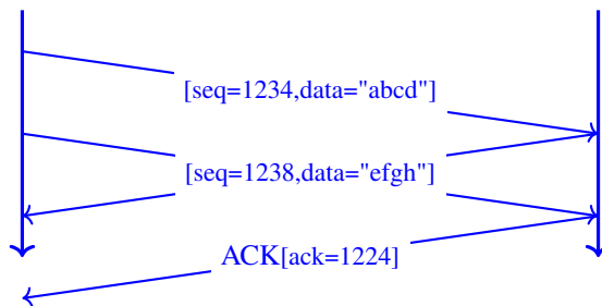
Fig. 2.3: TCP Reliable data transfer
